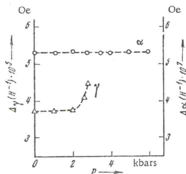
Fig. 3. Oscillation periods of the sound absorption coefficient in relation to the pressure.
